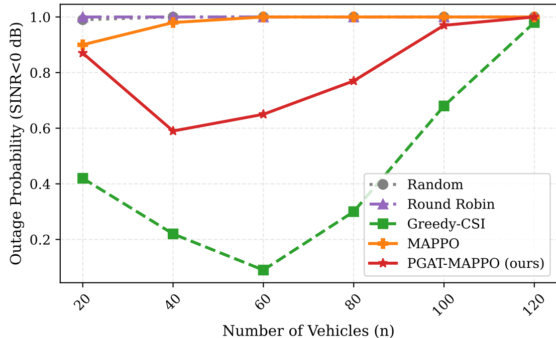
Outage Probability vs. Number of Vehicles
