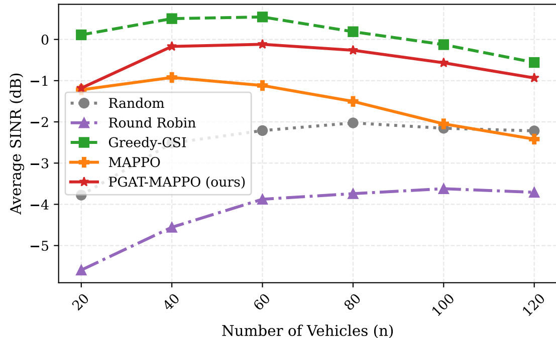
Average SINR vs. Number of Vehicles
