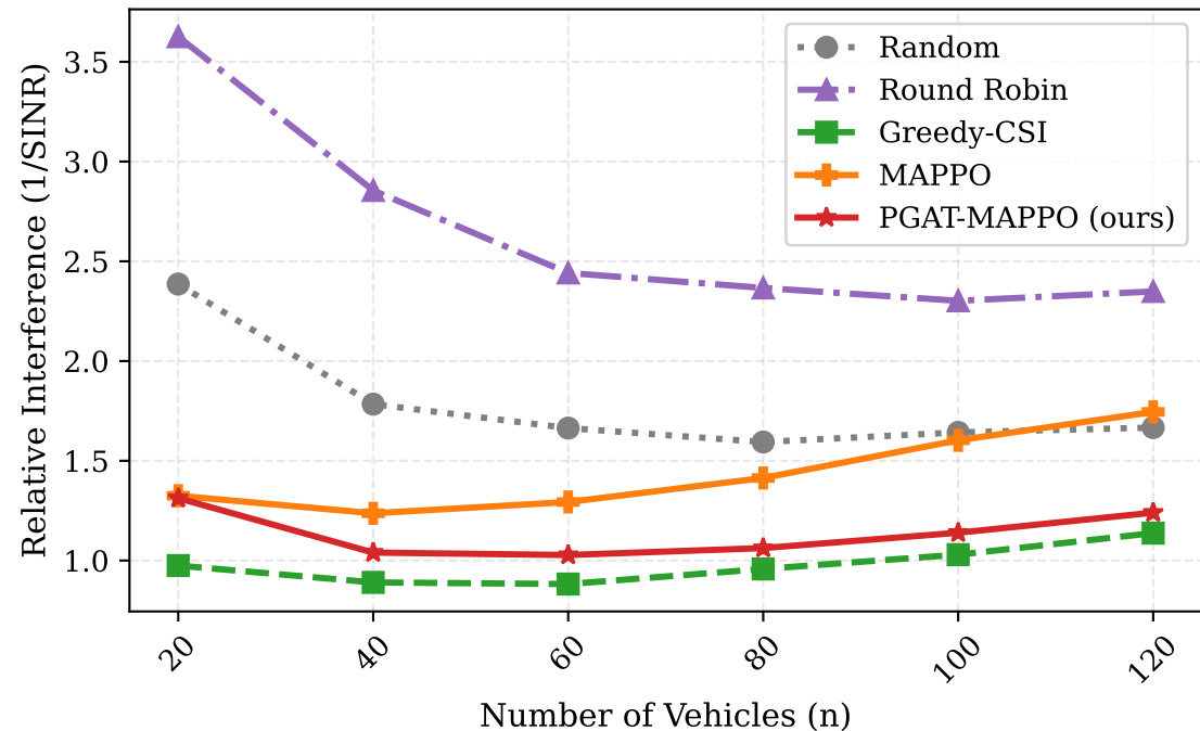
Interference vs. Number of Vehicles
