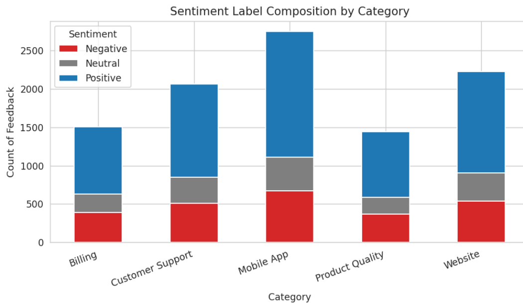
Fig 3.2 – Sentiment Composition by Category (Stacked Bar)
