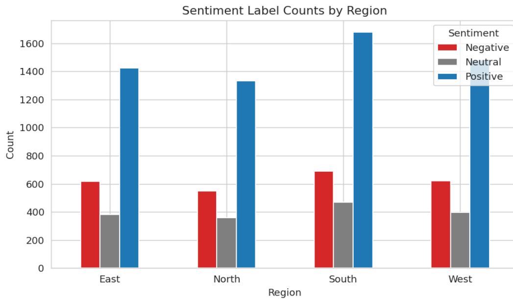
Fig 4.1 – Sentiment Label Counts by Region (Grouped Bar)
