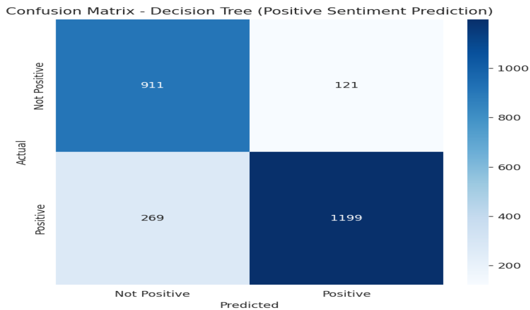
Fig 10.2 – Confusion Matrix – Decision Tree (Sentiment Prediction)
