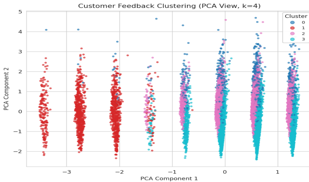
Fig 10.4 – Customer Feedback Clustering (PCA View, k=4)
