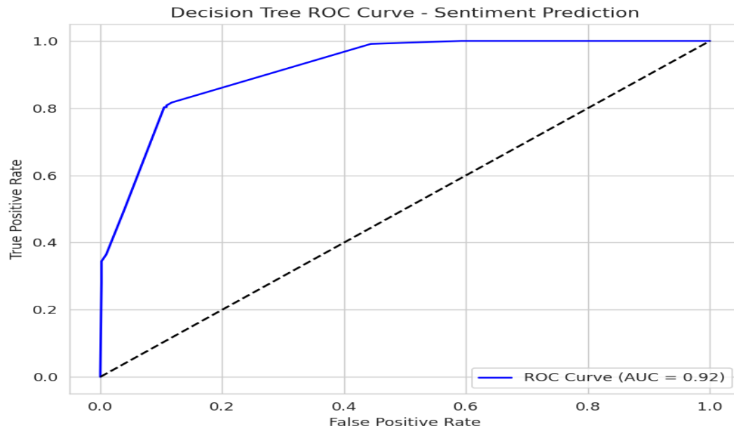
Fig 10.3 – Decision Tree ROC Curve – Sentiment Prediction
