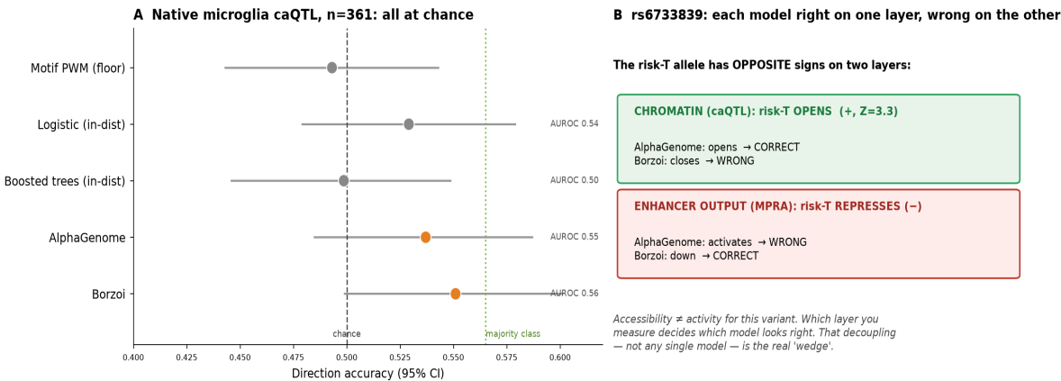
Figure 1. Direction accuracy on the native human-microglia caQTL test set ( n = 361 ). Both frontier models (AlphaGenome, Borzoi), motif floor baselines, and in-distribution controls fall at or below the majority-class baseline (0.565); error bars are 95% bootstrap confidence intervals.
