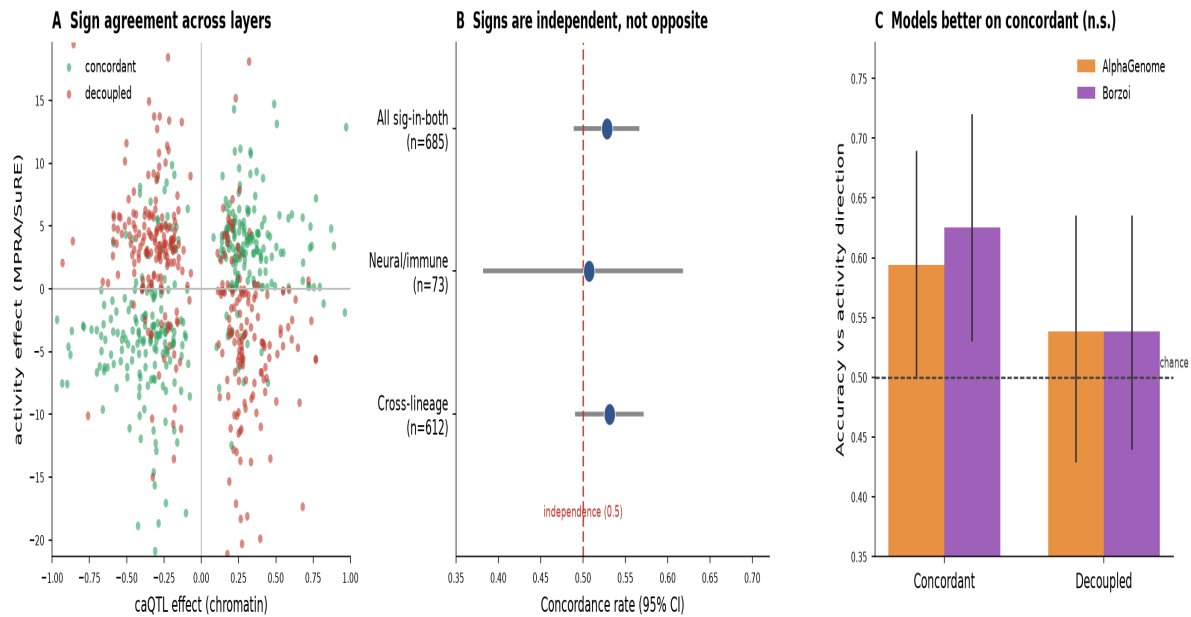
Figure 2. Layer-decoupling at scale (caQTL versus MPRA/SuRE enhancer activity). Sign agreement by stratum, robustness to dropping estimate-derived datasets, and model accuracy stratified by concordant versus decoupled variants.
