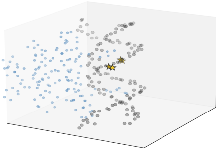
Figure 4. Boltz-2 co-fold of the MEF2A dimer on the BIN1 enhancer, shown in a shared orientation for the reference (non-risk C) and alternate (risk T) alleles. Both complexes are high-confidence (interface pTM 0.978); the risk allele forms a tighter protein-DNA interface (+12.5% contacts within 4 Å). The rs6733839 site is marked.
