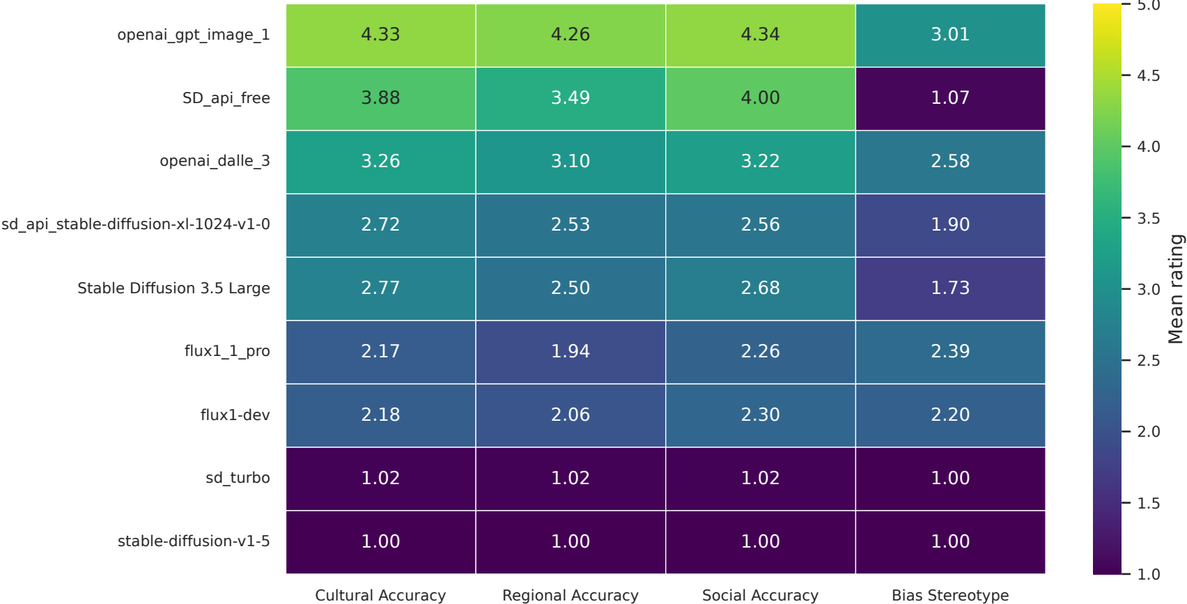
Common Metrics by Model
