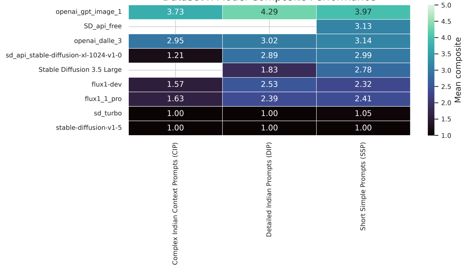
Dataset x Model Composite Performance
