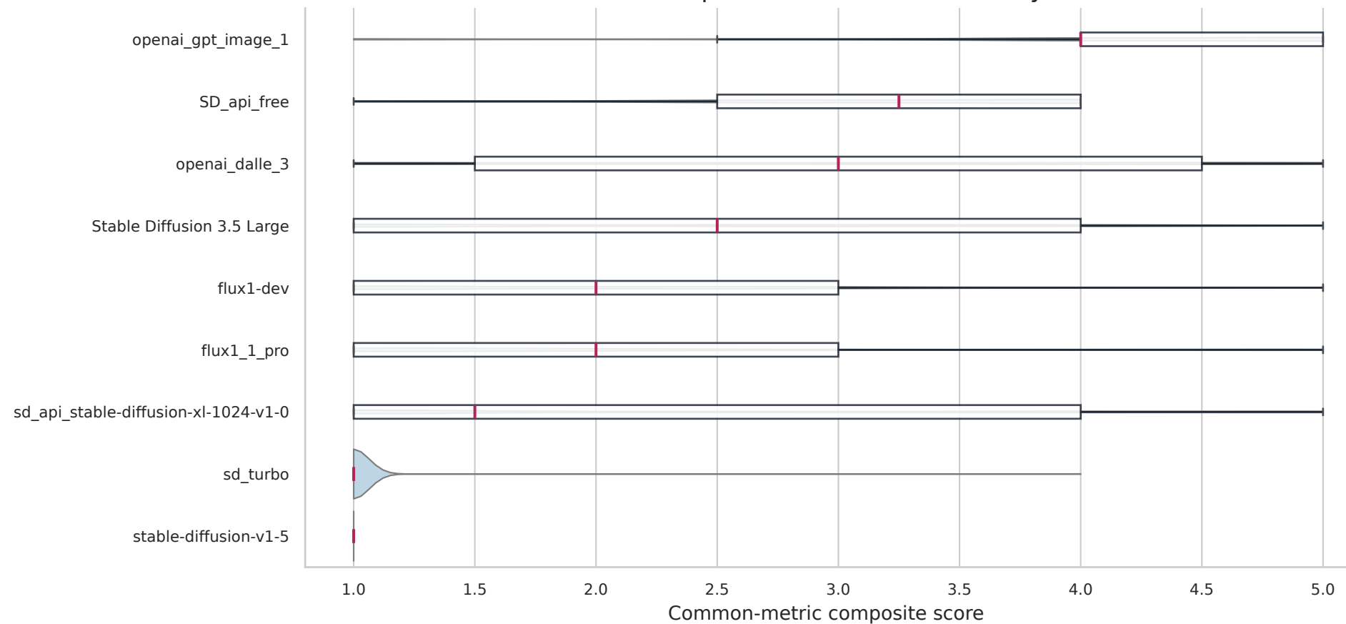
Common Composite Score Distribution by Model
