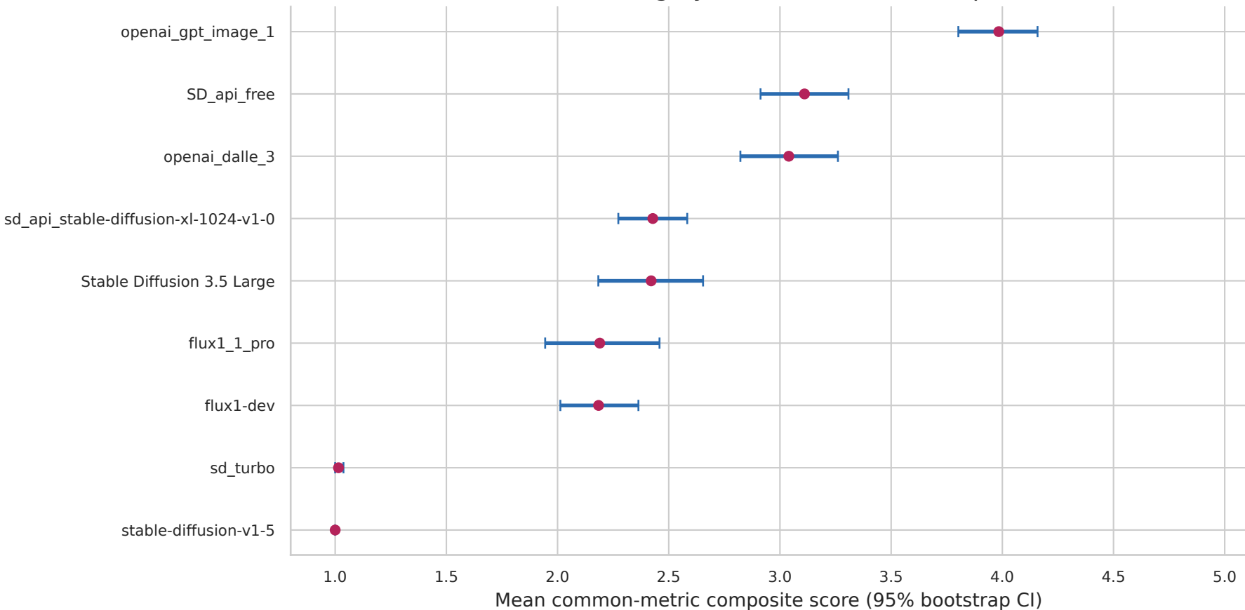
Model Ranking by Common-Metric Composite
