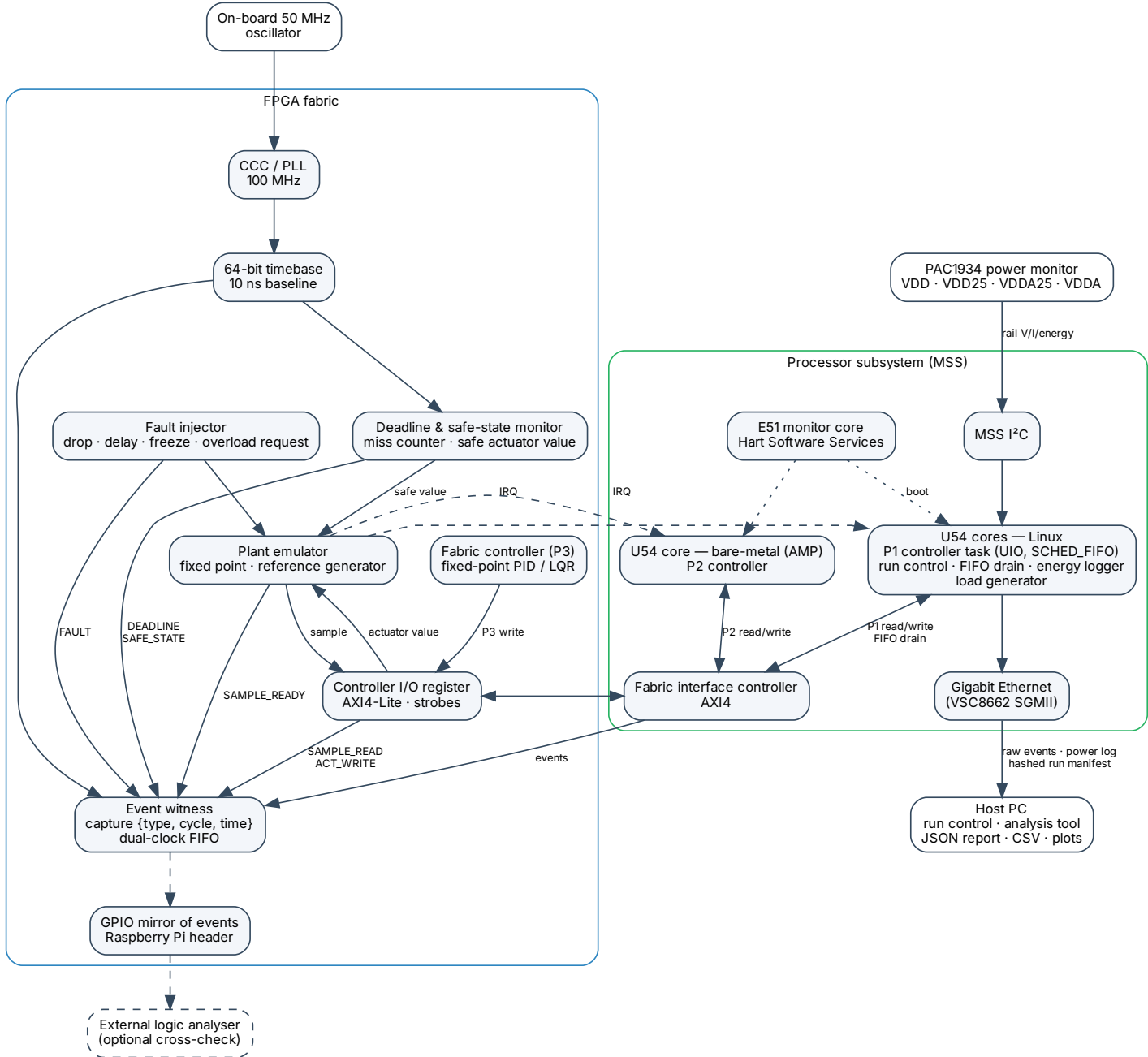
Loop Timing Witness — system block diagram (PolarFire SoC Icicle Kit, MPFS250T)
