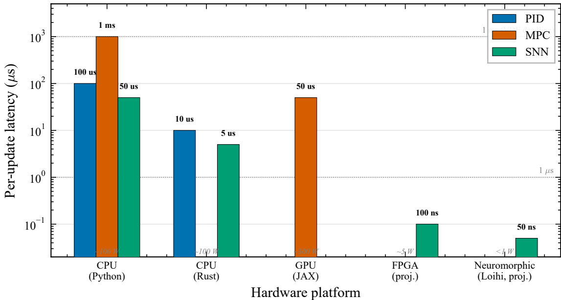
Controller latency across hardware platforms
