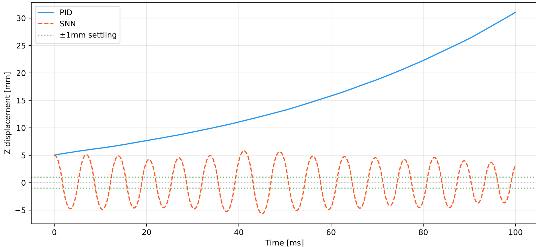
Plant Uncertainty: \gamma+20\% , gain -30\%
