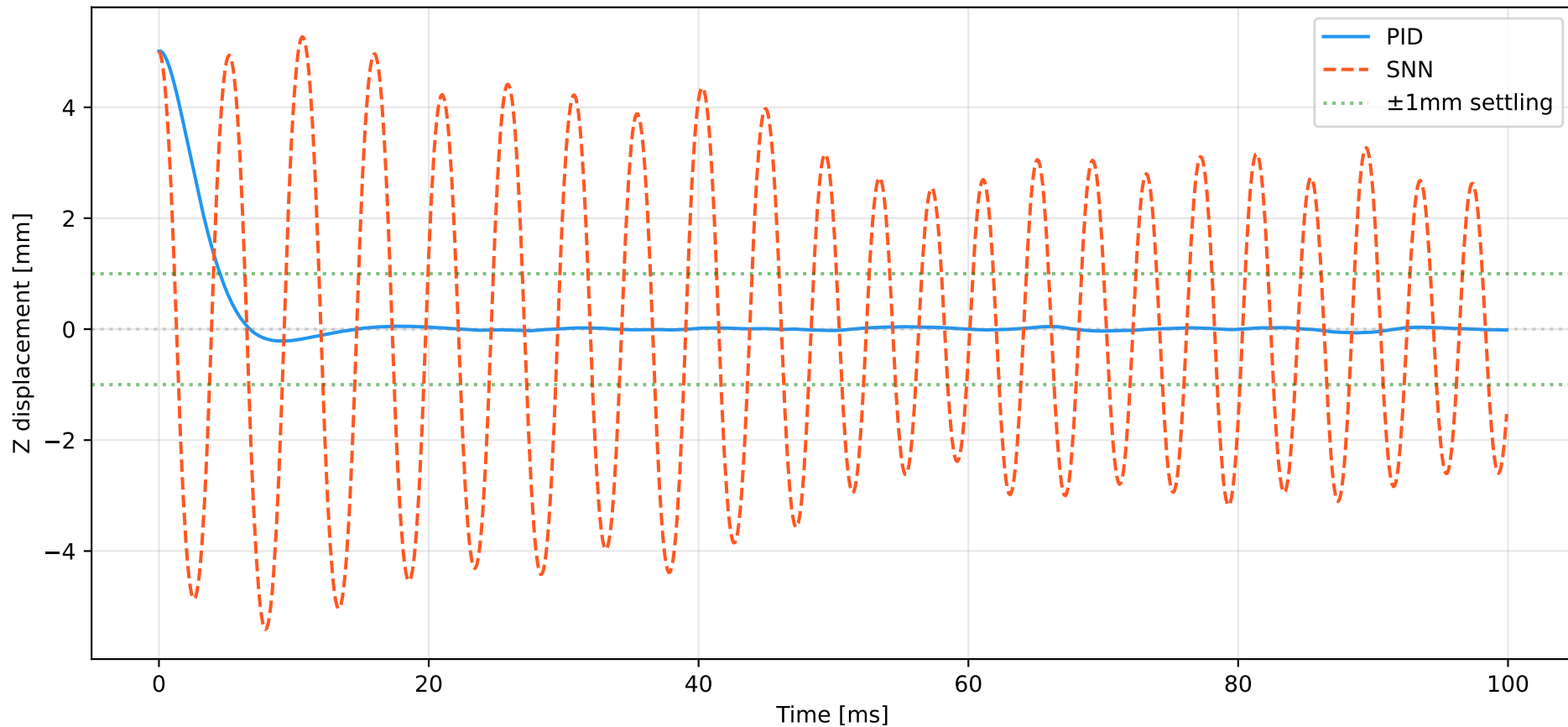
Step Response: 5mm Initial Displacement
