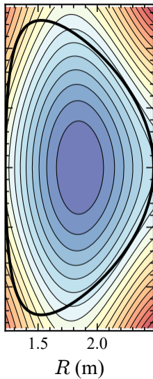
(b) Reconstructed (5 LM iter.)
