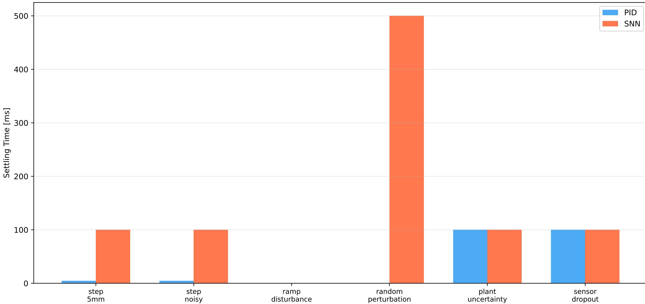
Settling Time Comparison: PID vs SNN
