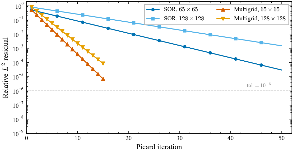
Picard iteration convergence: SOR vs multigrid
