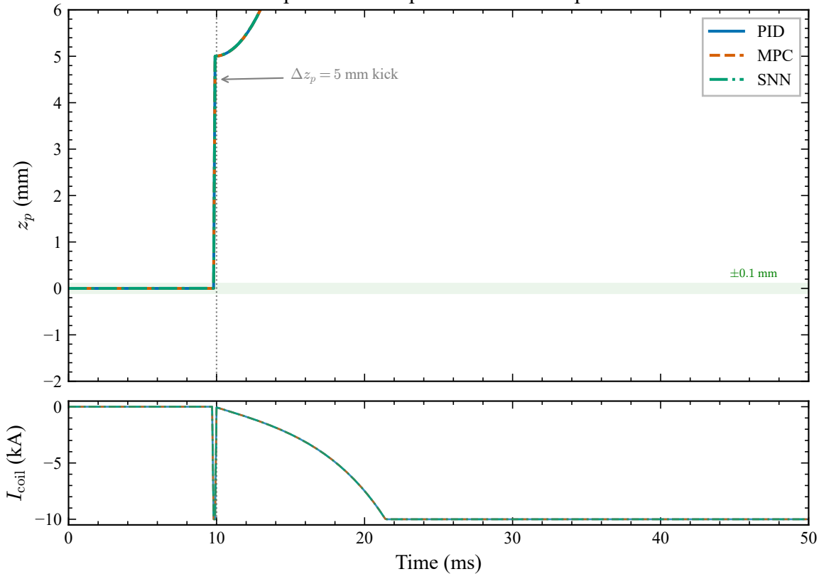
Vertical displacement response to 5 mm step disturbance
