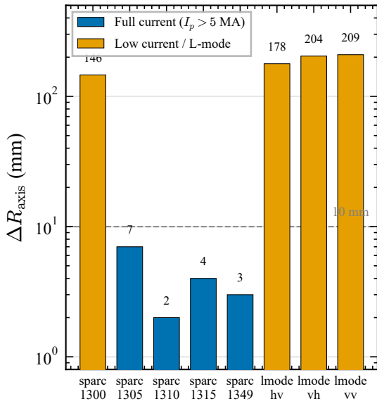
(a) SPARC magnetic axis error
