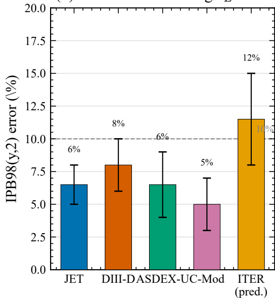
(b) Confinement scaling \tau_E error
