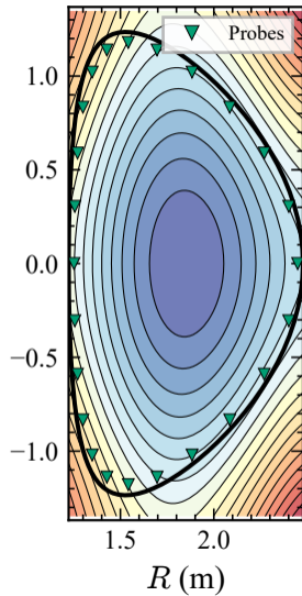
(a) Target equilibrium
