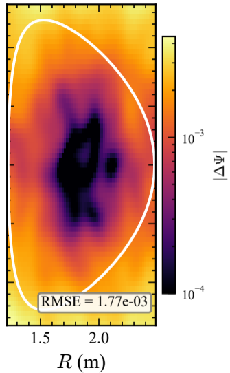
(c) Residual |\Delta\Psi|
