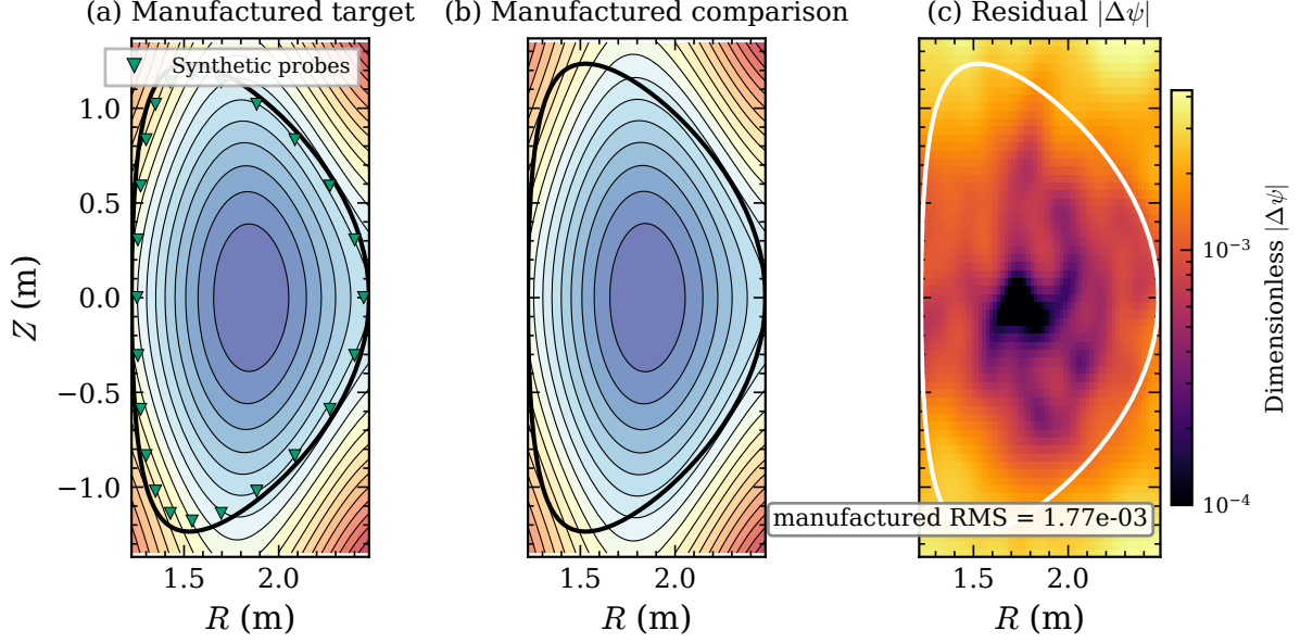
Figure 1: Deterministic manufactured inverse-reconstruction illustration. Target flux, perturbed comparison flux and residual are generated from synthetic probe locations. This figure is not experimental validation.
