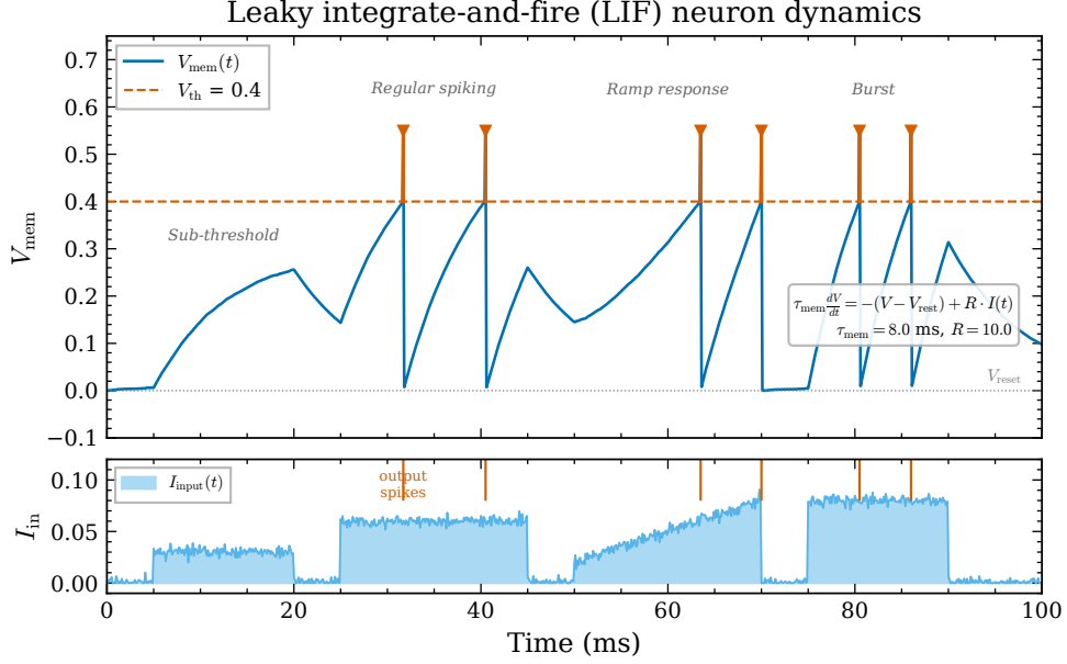
Figure 3: Pedagogical LIF response generated by the paper-local script.
