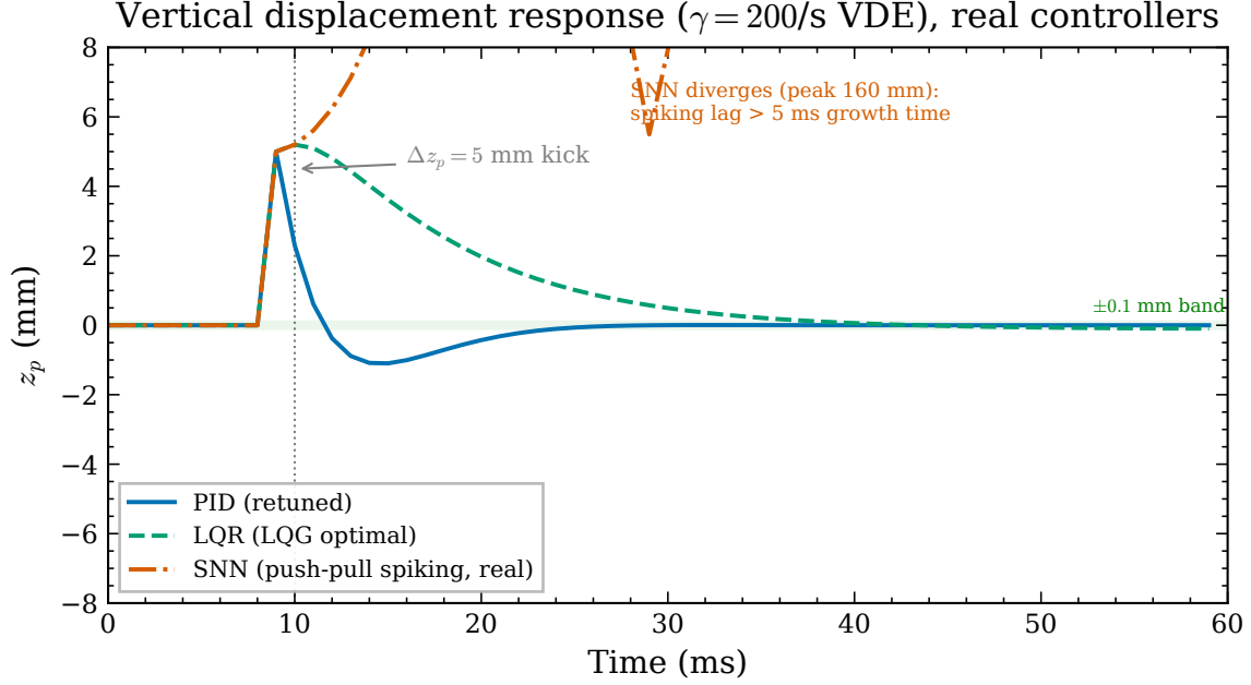
Figure 4: Same-plant response of the implemented controllers. The SNN curve leaves the displayed range and peaks near 160 mm. This is a reduced-order numerical experiment, not a tokamak discharge.
