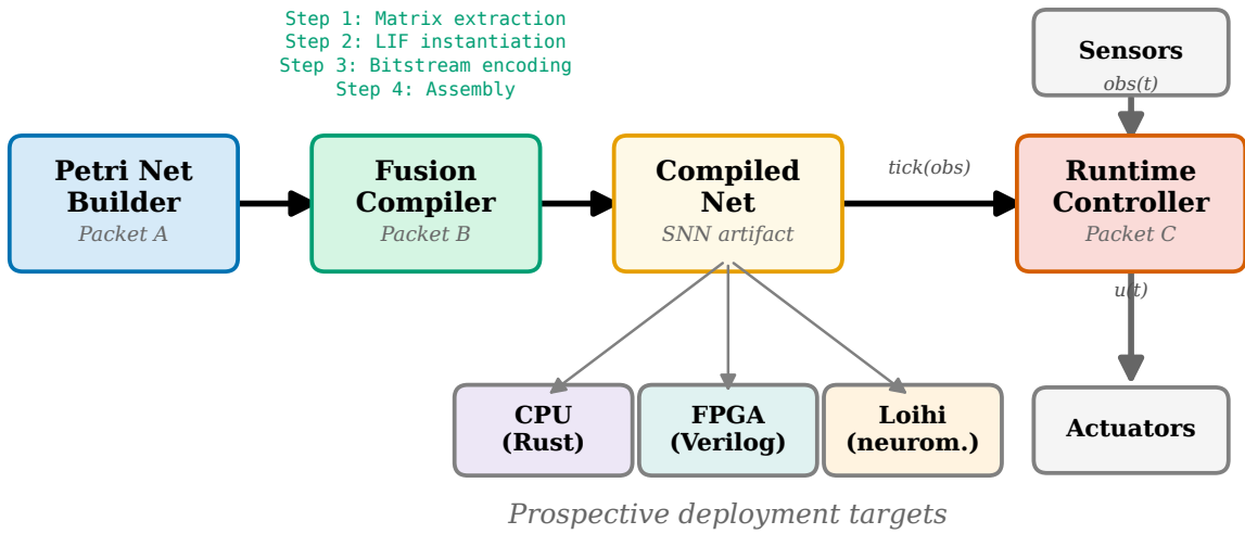
Figure 2: Software compilation path from policy graph to runtime artefact. Hardware targets are prospective; this draft reports software execution.
