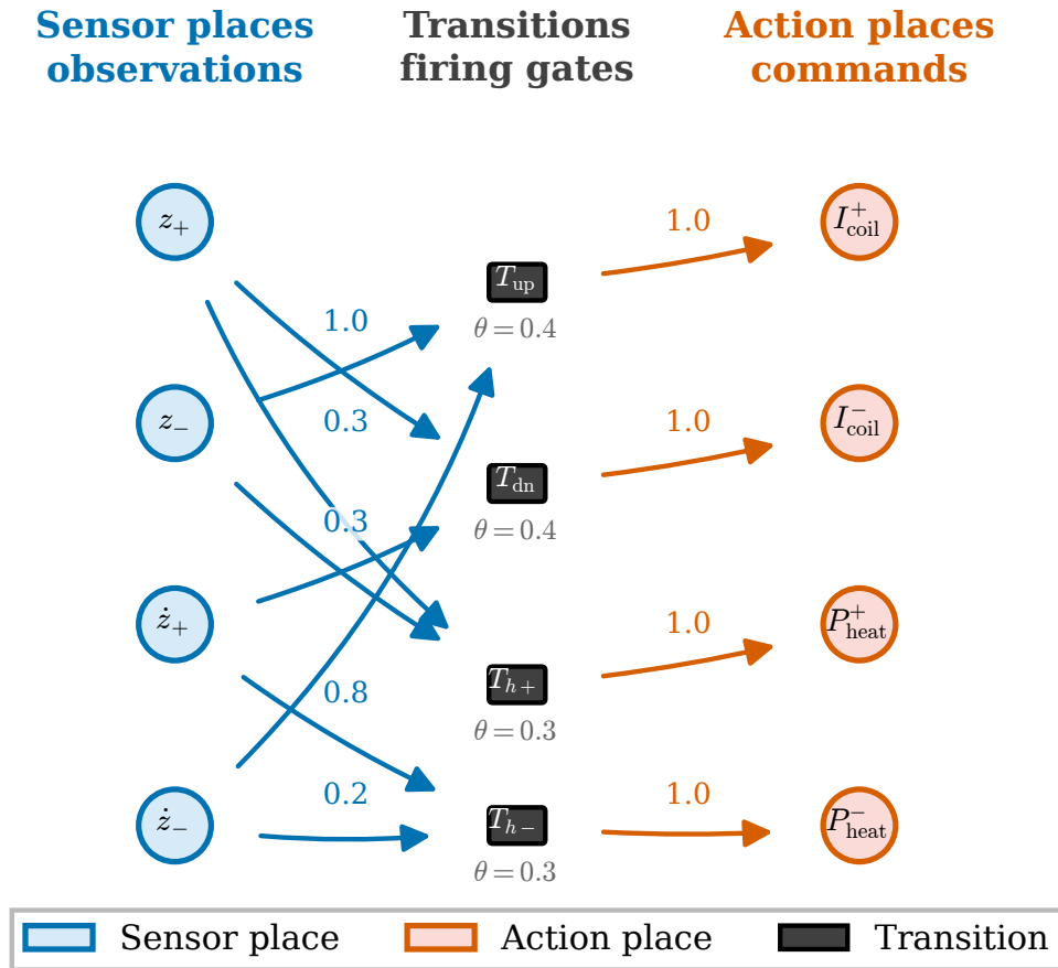
Figure 1: Eight-place, four-transition Petri-net policy used by the compiler fixture. The diagram describes software state flow; it is not a facility safety case.
