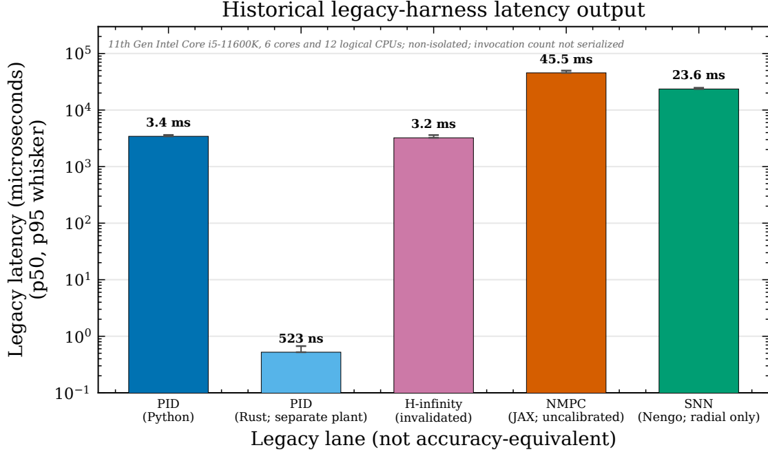
Figure 5: Historical legacy-harness output, p50 with a p95 whisker. The source values are preserved exactly, including the invalidated H-infinity lane. Different plant/action paths and an unknown invocation count prohibit a current controller ranking.
