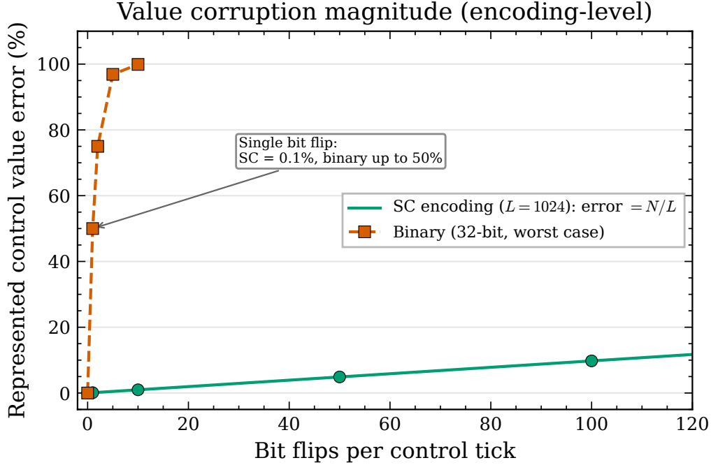
Figure 6: Analytical encoding-error illustration. The plotted arrays are not irradiation measurements and do not establish device-level fault tolerance.
