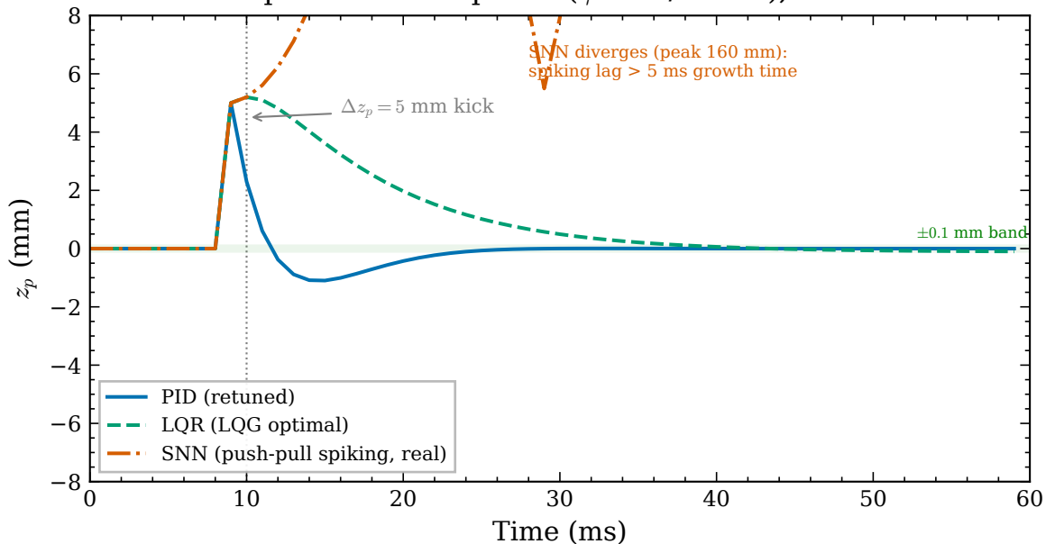
Vertical displacement response ( \gamma = 200/\text{s} VDE), real controllers
