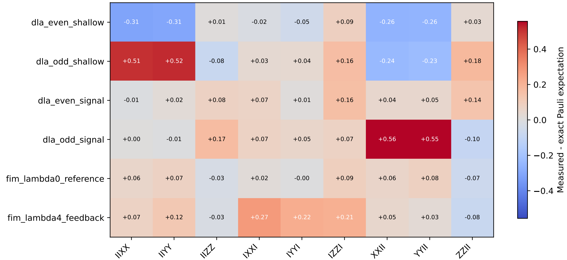
Phase 3 reduced-Pauli deviations on ibm_marrakesh
