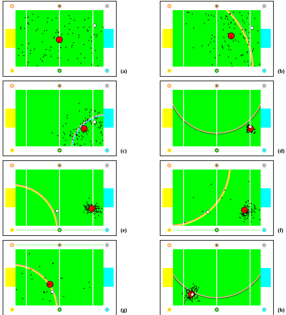
Figure 8.15 Mont Carlo localization with random particles. Each picture shows a particle set representing the robot's position estimate (small lines indicate the orientation of the particles). The large circle depicts the mean of the particles, and the true robot position is indicated by the small, white circle. Marker detections are illustrated by arcs centered at the detected marker. The pictures illustrate global localization (a)–(d) and relocalization (e)–(h).
