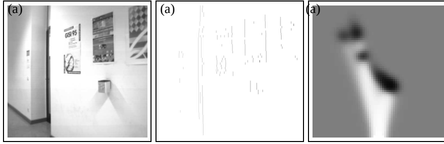
Figure 9.5 Estimation of occupancy maps using stereo vision: (a) camera image, (b) sparse disparity map, (c) occupancy map by projecting the disparity image onto the 2-D plane and convolving the result with a Gaussian.
