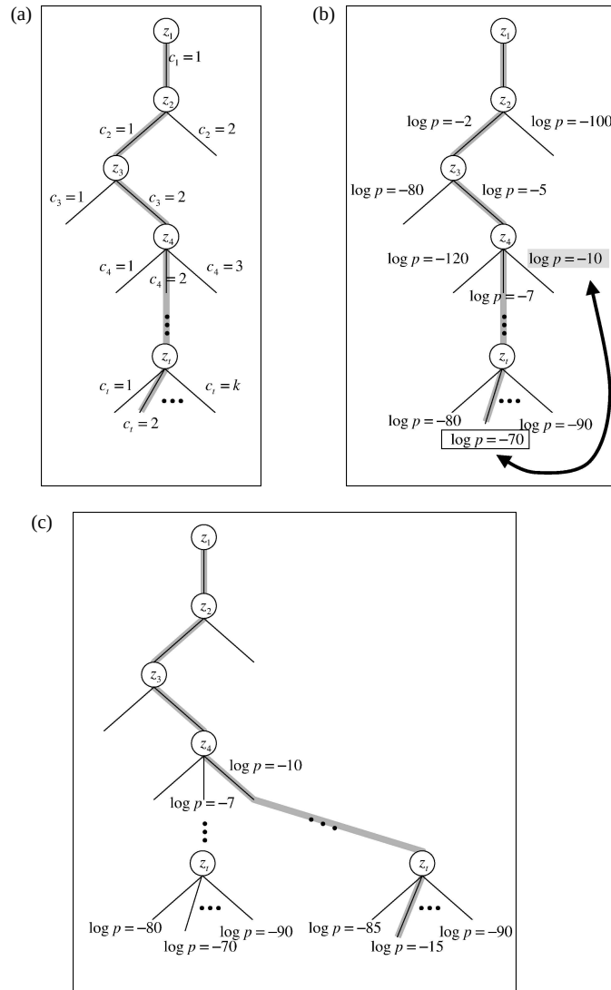
Figure 12.17 (a) The data association tree, whose branching factor grows with the number of landmarks in the map. The tree-based SEIF maintains the log-likelihood for the entire frontier of expanded nodes, enabling it to find alternative paths. (c) Improved path.
