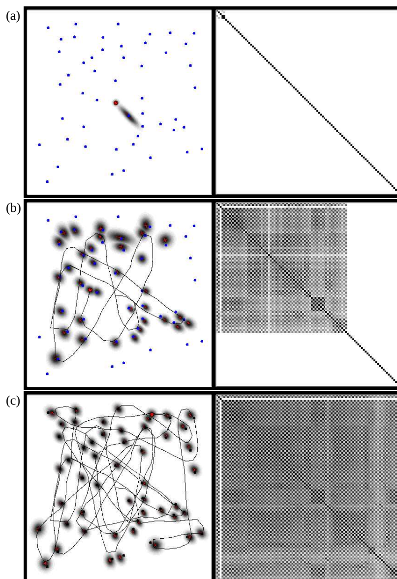
Figure 10.2 EKF SLAM with known data association in a simulated environment. The map is shown on the left, with the gray-level corresponding to the uncertainty of each landmark. The matrix on the right is the correlation matrix, which is the normalized covariance matrix of the posterior estimate. After some time, all x - and all y -coordinate estimates become fully correlated.
