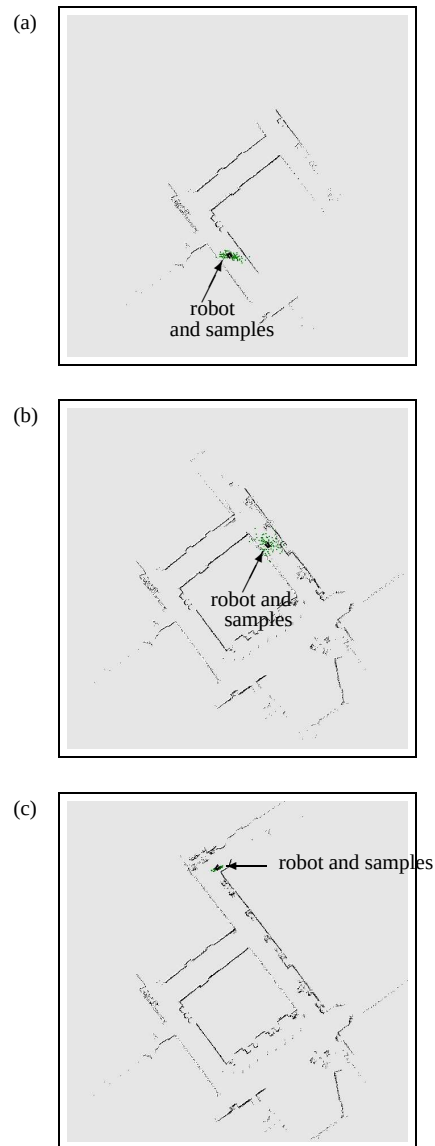
Figure 14.3 Mapping cyclic environments using particle filters for posterior pose estimation. The dots, centered around the robot, indicate the posterior belief which grows over time (a and b). When the cycle is closed as in (c), the map is revised accordingly and the posterior becomes small again.
