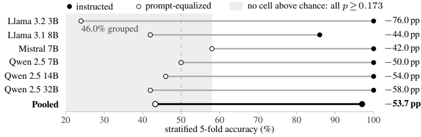
Figure 2: EXP-R1c: the pre-registered collapse, on every target. Prediction (§2.1): removing the instruction asymmetry removes any signal attributable to E or C . Test : prompt equalization, pre-registered before any cell was collected, on 50 disjoint claim pairs and 16 independently worded probes ( n = 50/\text{cell} ; instructed every p = 0.001 ; Appendix Table 37). The shaded band spans the equalized cells; points below the dashed chance line mark a degenerate probe channel (0–2 of 16 dimensions varying)—absence of a usable signal, not inverted discrimination (3B’s 24.0% is stratified 5-fold; claim-pair-grouped folds give 46.0%).
