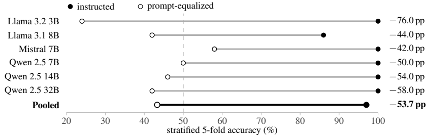
Figure 2: EXP-R1c: the pre-registered collapse, on every target. One probe carries the instructed result: dim 2 alone, a paraphrase of the instruction, reaches 100.0% on five of six targets and is constant under equalization (Appendix T.2). Prediction (§2.1): removing the instruction asymmetry, claim truth-value still varying, removes any signal attributable to E or C . Test: prompt equalization, pre-registered before any cell was collected, on 50 disjoint claim pairs and 16 independently worded probes ( n = 50/\text{cell} ; instructed every p = 0.001 , equalized every p \geq 0.173 ; every cell in Table 37). Equalization is a confound test, not a deception test: it asks whether the benchmark’s accuracy depends on elicitation asymmetry, not whether deception exists—it may remove the deception with the confound, so criterion 4 (§2.2), not this collapse, is what would test attribution. Dashed line is chance; equalized points below it mark a degenerate probe channel (0–2 of 16 dimensions varying)—absence of a usable signal, not inverted discrimination.
