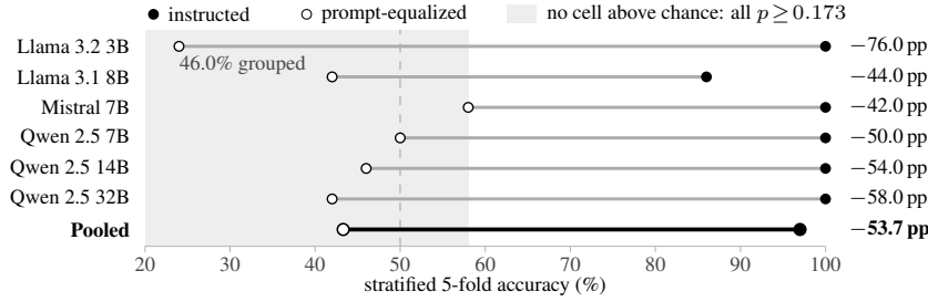
Figure 3: EXP-R1c: the pre-registered collapse, on every target. Prediction (§2.1): removing the instruction asymmetry removes any signal attributable to E or C . Test : prompt equalization, pre-registered before any cell was collected, on 50 disjoint claim pairs and 16 independently worded probes ( n = 50/\text{cell} ; instructed every p = 0.001 ; Appendix Table 37). The shaded band spans the equalized cells; points below the dashed chance line mark a degenerate probe channel (0–2 of 16 dimensions varying)—absence of a usable signal, not inverted discrimination (3B’s 24.0% is stratified 5-fold; claim-pair-grouped folds give 46.0%).
