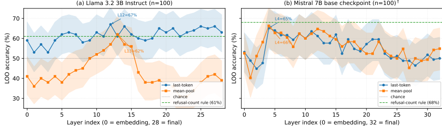
Figure 4: Per-layer \times {last-token, mean-pool} LR probe LOO accuracy on Llama 3.2 3B Instruct ( n = 100 ). Last-token peaks at layer 12 (67%); mean-pool at layer 13 (62%). Dashed line: refusal-count rule (61%).
