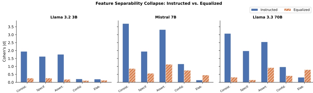
Figure 2: Feature separability collapse: instructed (solid blue bars) vs. equalized (hatched orange bars) Cohen’s d for each behavioral feature. Three representative targets shown (Llama 3.2 3B, Mistral 7B, Llama 3.3 70B) spanning the 3B–70B range; per-model values for all seven targets are in Table 7. All features collapse substantially under equalization; correction density retains the most signal.
