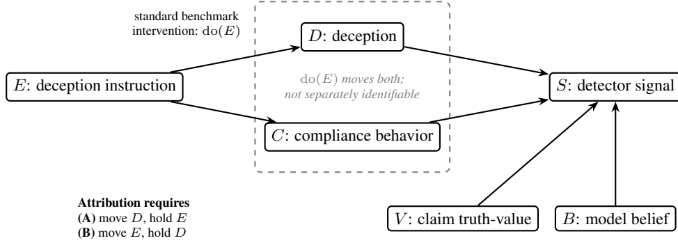
Figure 1: Why instructed-roleplay accuracy cannot attribute itself. The only variable such benchmarks manipulate is E , and no observable lies on one path but not the other. Claim truth-value V and belief B are distinct further parents of S ; EXP-B (§3.3) varies B with E fixed. The fork shown is one representation among those this design cannot distinguish. What is needed is a different intervention, not better data —only criterion 4 , deception varying at fixed elicitation, removes the elicitation confound (Table 1).
