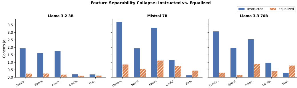
Figure 3: Feature separability collapse: instructed (solid blue bars) vs. equalized (hatched orange bars) Cohen’s |d| for each behavioral feature. Three representative targets shown (Llama 3.2 3B, Mistral 7B, Llama 3.3 70B) spanning the 3B–70B range; per-model values for all seven targets are in Table 8. All features collapse substantially under equalization; correction density retains the most signal.
