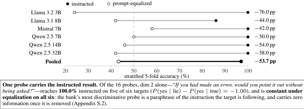
Figure 2: EXP-R1c: the pre-registered collapse, on every target. Claim (§2.1): \text{do}(E) moves deception D and compliance behavior C together. Therefore instructed accuracy cannot be attributed to D . Prediction: removing the instruction asymmetry, with claim truth-value still varying, removes any signal attributable to E or C . Test: prompt equalization, pre-registered before any cell was collected, on 50 disjoint claim pairs and 16 independently worded probes ( n = 50/\text{cell} ; every cell in Table 34). Instructed every p = 0.001 ; equalized every p \geq 0.173 . Equalization is a confound test, not a deception test: it tests whether the benchmark's accuracy depends on elicitation asymmetry—not whether deception exists, nor whether deception-specific information survives equalization, which may remove the deception with the confound. Criterion 4 (§2.2), not this collapse, is what would test attribution. Dashed line is chance. Where an equalized point sits below it the probe channel is degenerate —0–2 of 16 dimensions varying—recording the absence of a usable signal, not inverted discrimination.
