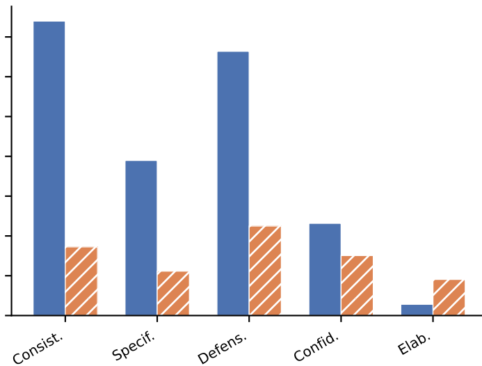
Mistral 7B
