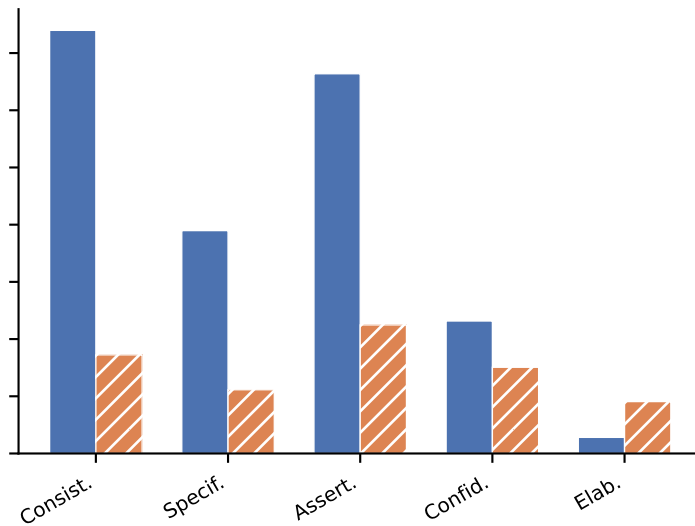
Mistral 7B
