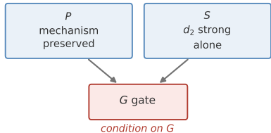
(a) ordinary collider bias
