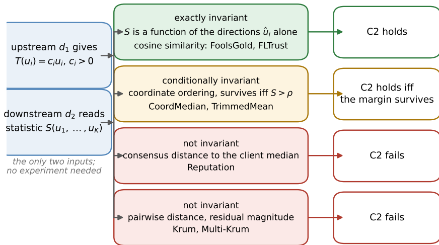
(a) What the criterion checks: invariance class of d_2 's statistic
