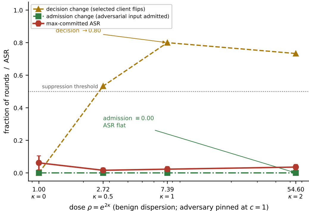
(a) Mode S, Krum: the statistic moves, admission does not
