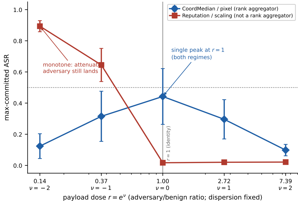
(b) Mode A: the payload dose isolates the two regimes
