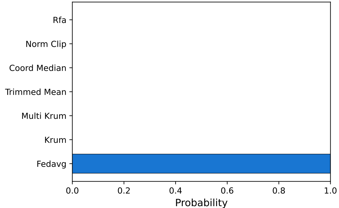
Server Mixed Strategy (NE)
