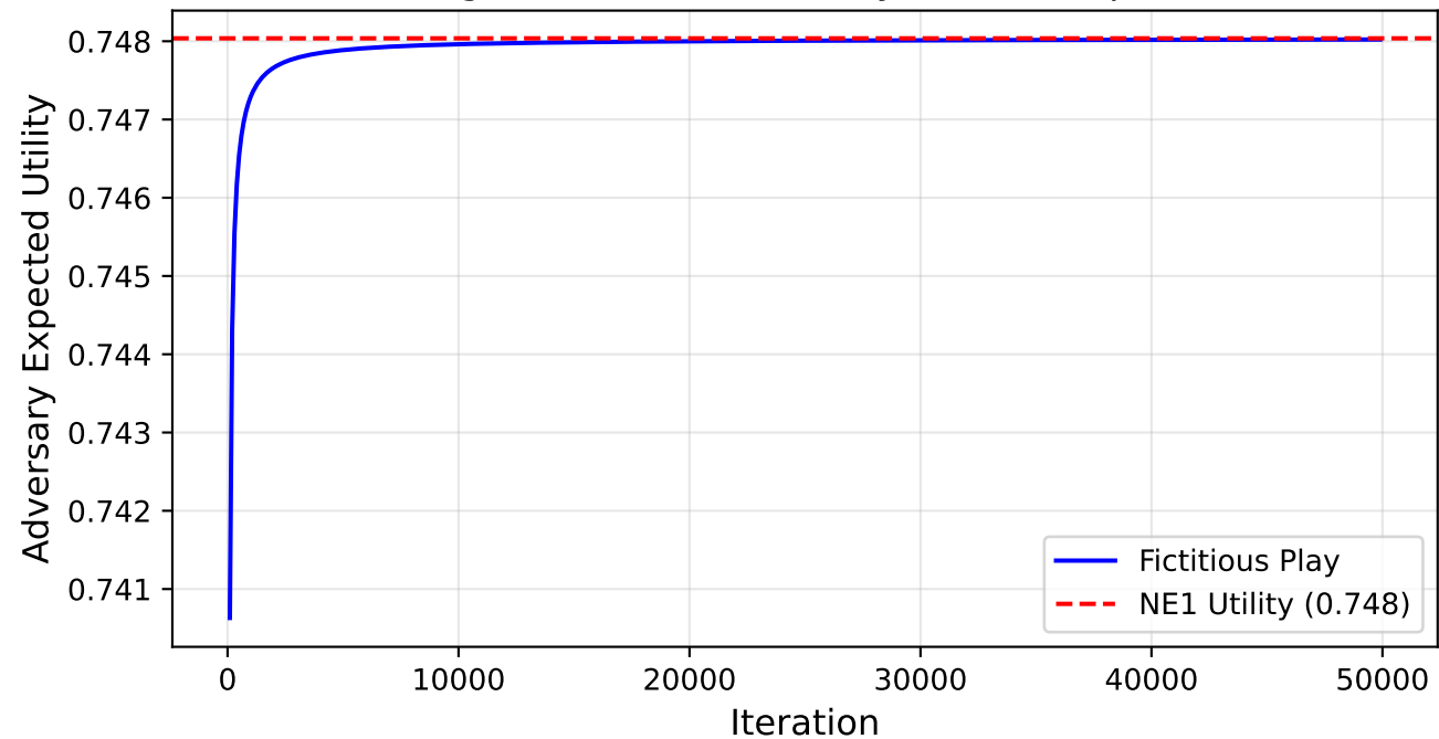
Convergence of Fictitious Play to Nash Equilibrium
