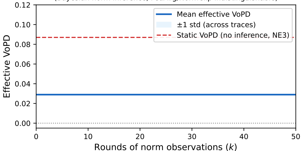
Inference-aware adversary: effective VoPD vs. observation rounds (Bayesian norm inference, FedAvg/NormClip indistinguishable)
