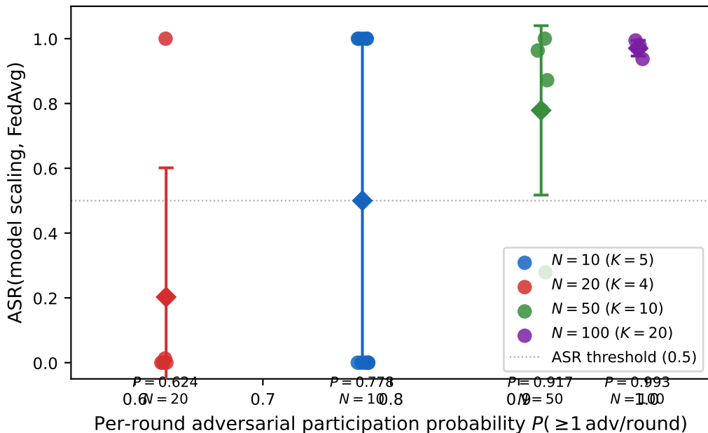
Per-seed ASR vs. adversarial participation probability (CIFAR-10, f = 0.2 , 4 \times 5 game; mean \pm std shown as diamonds)
