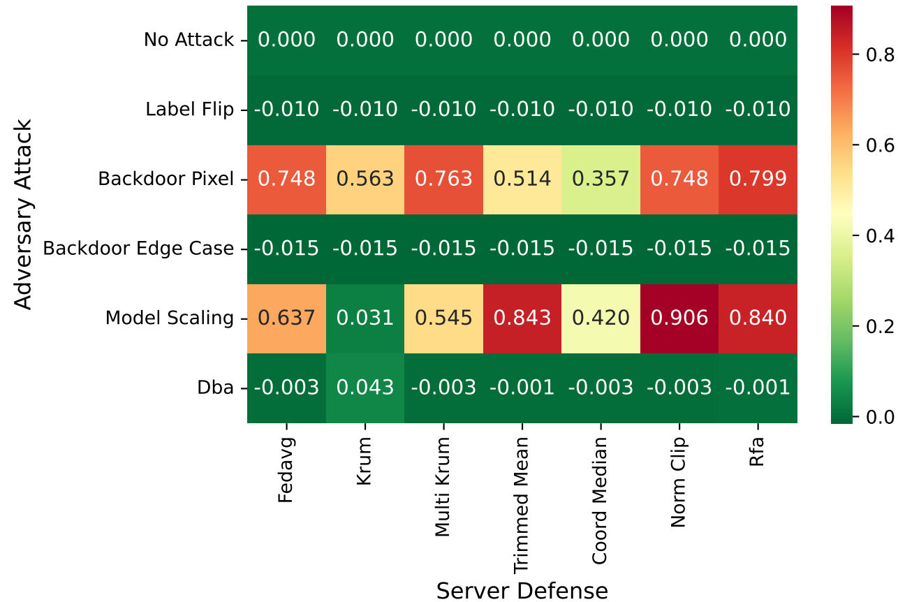
Adversary Payoff Matrix
