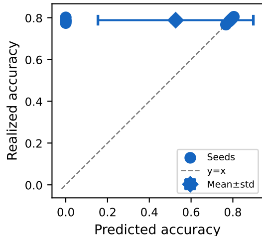
(a) No Attack (accuracy)
