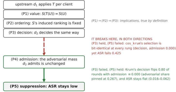
Figure A5: The preservation chain, and where it breaks. (P1) \Rightarrow (P2) \Rightarrow (P3) holds by definition; the (P3)–(P4) link breaks in both directions, and both witnesses come from the oracle intervention that pins every adversary’s coefficient and so closes Lemma 2’s attenuation channel by construction (§E.2). The pooled statistic-level prediction we had frozen is separately rejected by a pre-registered ladder ( \rho_s = +0.351 , one-sided p = 0.091 , 16 cells; §E), and a pre-registered replication in a different invariance class reproduces the negative but refutes the cross-arm admission ordering ( \Delta = +0.098 ; the pooled two-channel model stays unconfirmed, R^2 = 0.239 over 26 cells), so admission is a direction, not a validated predictor . Every number in the figure and in this caption is recomputed from the scoring scripts’ own JSON and printed by story_chain.figure.py .
