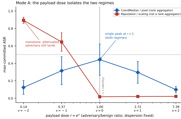
Figure A6: Mode A, the payload dose: the two mechanism-preserving regimes, and where they hold. With dispersion fixed and only the adversary/benign weight ratio r swept, coordmedian (a rank aggregator, the case Theorem 9's regimes are stated over) is single-peaked at r=1 as the theorem predicts (over-attenuated adversaries carry no payload, over-amplified ones are discarded) while reputation is monotone, off-spec and refuted for that shape. Mode A is the \Delta_c -swept companion to Mode S's \Delta_c -pinned design (Proposition 13); Mode S itself is Figure A5. Bars are Student- t 95% intervals; numbers recomputed per seed by analyze_targeted_dose.py .
