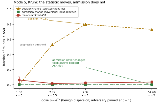
Figure A5: Mode S, the \Delta_c -pinned dose: Krum's statistic is disturbed, its admission of adversarial input is not, and suppression does not follow either. The instrument of §5 at the four rungs of the benign-dispersion dose, with every adversary's own weight pinned ( \Delta_c exactly 0 at every rung, so the attenuation channel is cut by construction rather than controlled for): the selected client flips in up to 0.80 of rounds, the admitted adversarial support changes in none of them, and max-committed ASR stays inside the pre-registered \pm 0.15 practical-equivalence margin. It is the \Delta_c -pinned companion to the \Delta_c -swept Mode A (Figure A6), and the same evidence Figure 1(a)'s middle annotation pools over four arms rather than Krum alone. Bars are Student- t 95% intervals, n=5 ; numbers recomputed per seed by analyze_targeted_dose.py .
