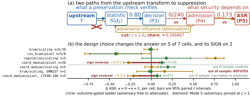
Figure 1: The paper in one figure. A preserved statistic is not preserved suppression. (a) The chain a preservation check reasons along, and the map of this paper’s vocabulary, at the levels of Def. 1: solid links hold by definition, each dashed link is marked \nRightarrow for not implied, and the lower arc is the attenuation channel Mode S cuts by construction. Its three numbers are three scopes, not one experiment (App. J), and the middle one pools four CIFAR-10 arms rather than Krum alone. (b) Seven cells, one contrast each, estimated both ways (App. D.3): the design choice changes the answer on 5 of 7 and its sign on 2. Row labels carry n per cell, outcome-gated/Mode S where the two differ, and the four cells above the dashed rule are training data for a since-withdrawn rule rather than evidence for it (Table A10). The Mode S dose evidence is Fig. A5.
