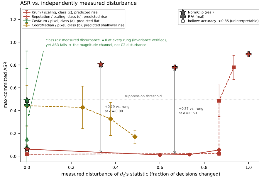
Figure A4: Why a transform’s flip rate is not a sufficient statistic for what it does. ASR against the independently measured disturbance of each arm’s own statistic ( n=5 , Student-t 95% intervals), the abscissa fixed before the freeze. Stars and crosses are the two real upstream transforms measured on these same ( d_2 , attack) cells (NormClip, RFA), placed at their own measured disturbance rate: at matched disturbance they sit +0.77 and +0.79 ASR above the synthetic curve, while their realized weight ratios (mean 3.61 and 11.93, maximum 4.90 and 17.38) fall inside the ladder’s span. The class-(a) arm’s four rungs coincide at disturbance exactly 0 (0/120 selections changed, maximum relative score drift 1.1 \times 10^{-4} ) and its ASR falls anyway: Lemma 2’s magnitude channel, not C2 disturbance.
