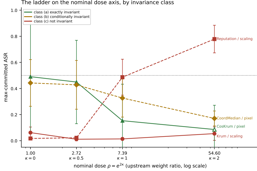
Figure A3: The ladder and its frozen predictions. The 16 cells on the nominal dose axis \rho = e^{2\kappa} ( n=5 per point, Student-t 95% intervals), coloured by Proposition 11 class. Of the two class-(c) arms whose statistics the framework’s fragility claim is stated over, only reputation rises; ASR falls with the dose in three of the four arms, against the predicted rises. Hollow markers fail the 0.35 clean-accuracy gate and are uninterpretable. Drawn by paper/figures/dose_response_figure.py , which recomputes every value from results/ and imports the arm construction from the scoring script so the two cannot diverge.
