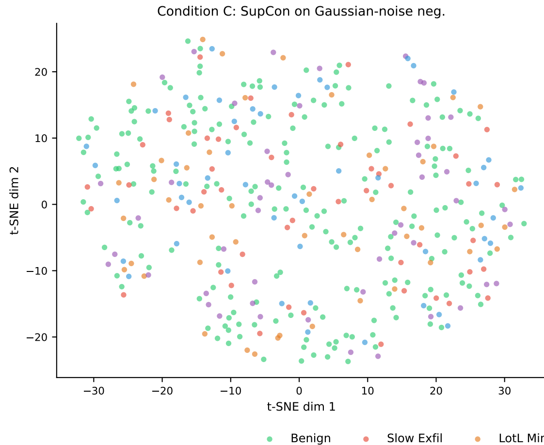
t-SNE projection of projection-head embeddings (stealth-95 test data)
