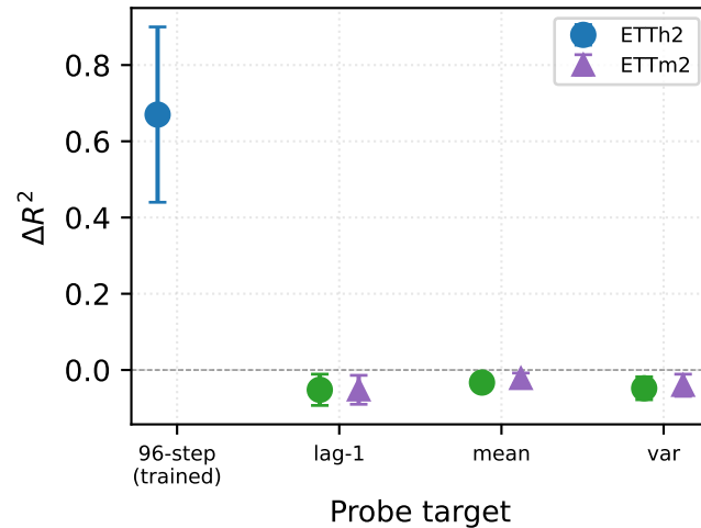
(c) Probe asymmetry ( n = 10k )
