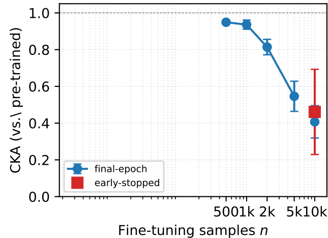
(a) Geometric drift
