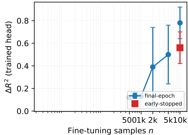
(b) Trained-head \Delta R^2 \uparrow
