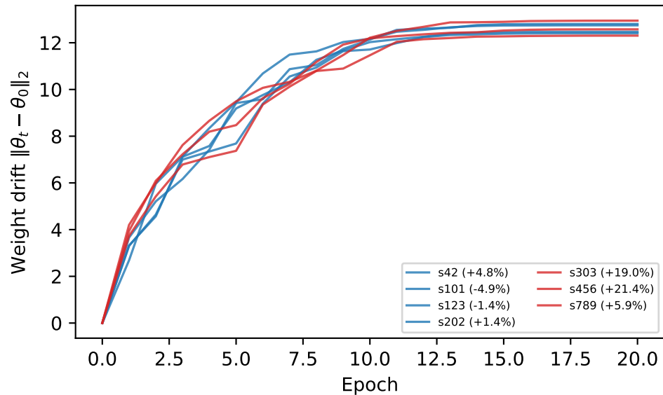
Weight drift trajectory, n = 5,000
