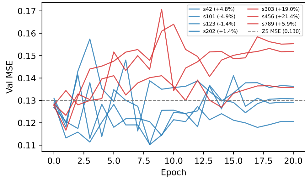
Val MSE trajectory, n = 5,000
