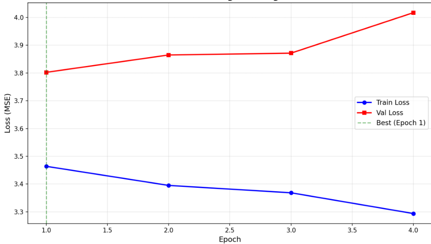
Moirai Fine-Tuning: Training Curves
