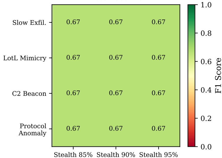
Best Baseline
