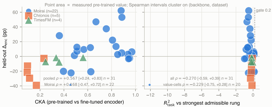
Figure 6: Neither drift nor measured pre-trained value orders the encoder intervention. Both panels share y = \text{held-out } \Delta_{\text{enc}} (positive = freezing the encoder did better). Point area is proportional to the graded value score in both panels, so the left panel answers the objection visually: if drift predicted the outcome wherever there was something to lose, the large points would trend and the small ones would scatter. Backbone is encoded by colour and marker because CKA is not comparable across architectures, which is why the pooled left-panel interval must not be read as a within-backbone one. Drawn by paper_8/fig_value_axis.py from results/value_axis.json ; the script asserts its own counts against that file and fails rather than drawing a figure that disagrees with this text.
