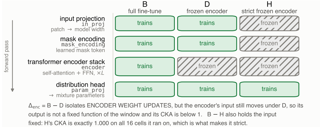
Figure 4: Where the freeze boundary falls, module by module. Green boxes are parameters the optimiser may move; hatched boxes are held at their pre-trained values. The grid is transcribed from the requires_grad assignments in scripts/finetune_forecasting.py . Two of our seven survivors change the sign of \Delta_{\text{enc}} between D and H (Table 12), so which of these columns a paper means by “we froze the encoder” is not a detail.
