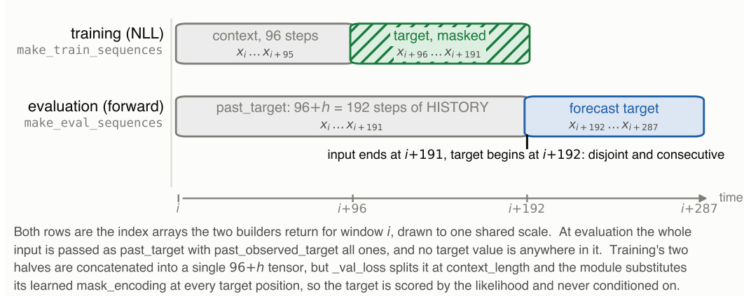
Figure 2: Which timesteps Moirai is given, and which it is asked to predict, at h=96 ; h=192 is the same layout with h substituted. Both rows are the index arrays that make_train_sequences and make_eval_sequences return for window i , drawn to one shared scale. At evaluation the model input is the 96+h steps preceding the forecast window and the target is the h steps strictly after it: the two are disjoint and consecutive, so no target value reaches the model. The figure is generated from those functions’ output and asserts that disjointness at draw time.
