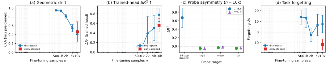
Figure 3: Cost-benefit dynamics on Moirai-Small/ETTh2 (condition B, h=96 ). (a) CKA decays monotonically with n (final-epoch vs. early-stopped markers); (d) forgetting is non-monotonic and protocol-dependent. Panels (b) and (c) plot the linear-probe \Delta R^2 statistic and its sign asymmetry, both retracted (§A29.4); they are reproduced unaltered as a record of the withdrawn analysis and support no claim here. The dissociation this figure is cited for is the contrast between (a) and (d): drift monotone in n , outcome not.
