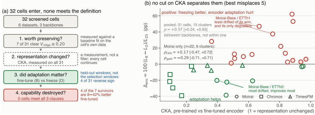
Figure 1: The whole paper. (a) The four layers of §3 as a funnel over the 31 cells that carry a selection-split gate: CKA filters none of them, and no cell meets either form of the degradation definition. (b) The same cells as CKA against held-out \Delta_{enc} (positive = freezing better): measured drift does not reliably predict the value of encoder adaptation , and no cut on CKA separates the cells adaptation helped from the cells it hurt. The labelled pairs are the paper’s running example: Moirai-Base’s two least drifted cells are its only two that degrade, and its two most drifted improve the most (§6). Filled markers clear the gate; both \rho are clustered by dataset×horizon, and only Moirai has enough cells to ask within one backbone (Appendix A27).
