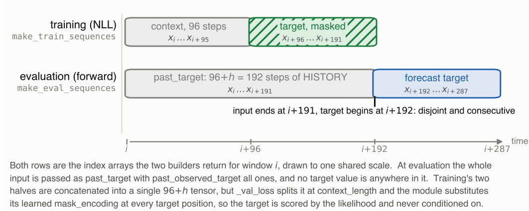
Figure 2: Which timesteps Moirai is given, and which it is asked to predict , at h=96 ; h=192 is the same layout with h substituted. Both rows are the index arrays that make_train_sequences and make_eval_sequences return for window i , drawn to one shared scale. At evaluation the model input is the 96+h steps preceding the forecast window and the target is the h steps strictly after it: the two are disjoint and consecutive, so no target value reaches the model. The figure is generated from those functions’ output and asserts that disjointness at draw time.
