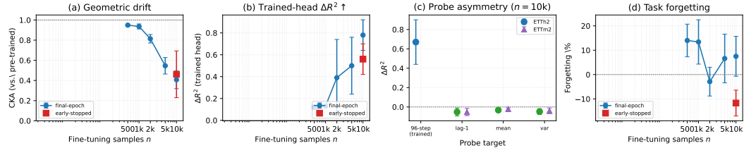
Figure 3: Cost-benefit dynamics on Moirai-Small/ETTh2 (condition B, h=96 ). (a) CKA decays monotonically with n (final-epoch vs. early-stopped markers); (d) forgetting is non-monotonic and protocol-dependent. Panels (b) and (c) plot the linear-probe \Delta R^2 statistic and its sign asymmetry, both retracted (§A29.4); they are reproduced unaltered as a record of the withdrawn analysis and support no claim here. The dissociation this figure is cited for is the contrast between (a) and (d): drift monotone in n , outcome not.
