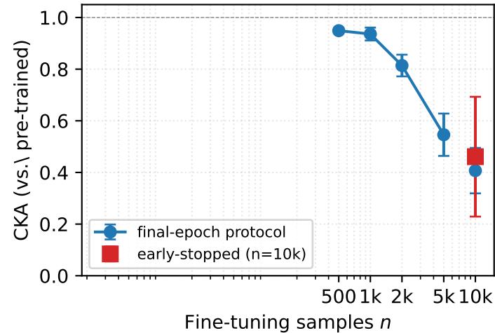
Geometric drift: CKA \downarrow
