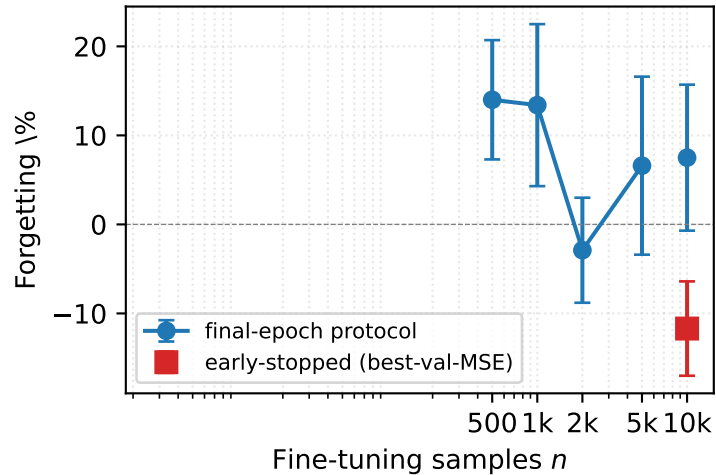
Task forgetting: non-monotonic
