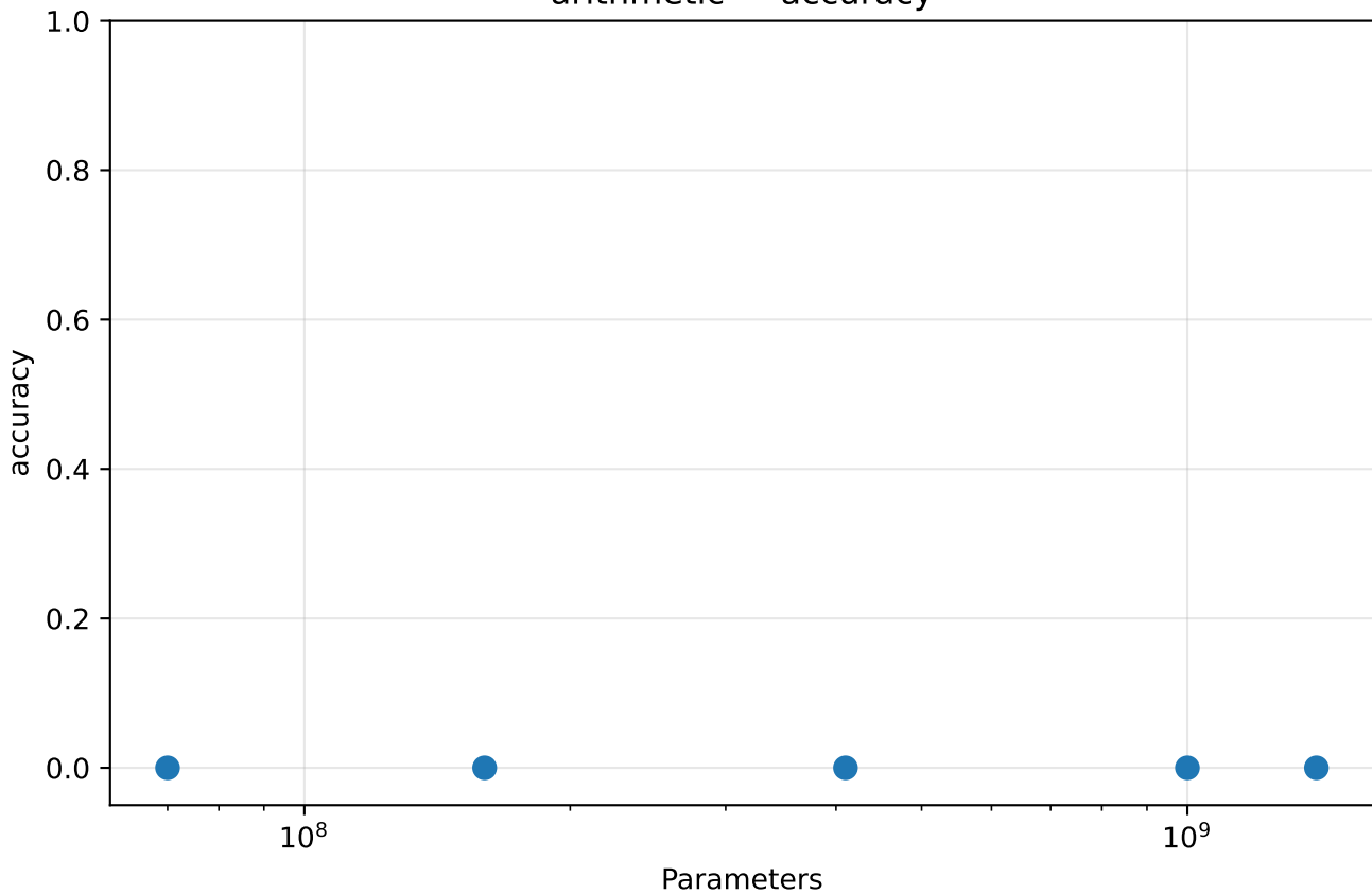
arithmetic — accuracy
