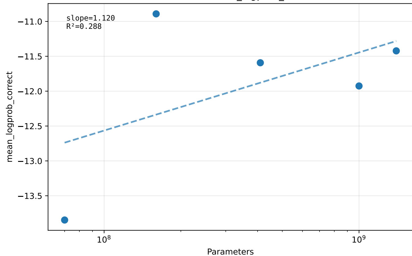
arithmetic — mean_logprob_correct
