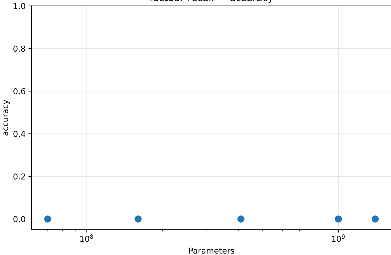
factual_recall — accuracy
