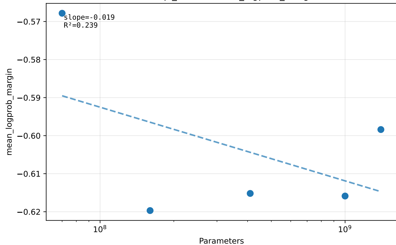
truthfulqa_mc1 — mean_logprob_margin
