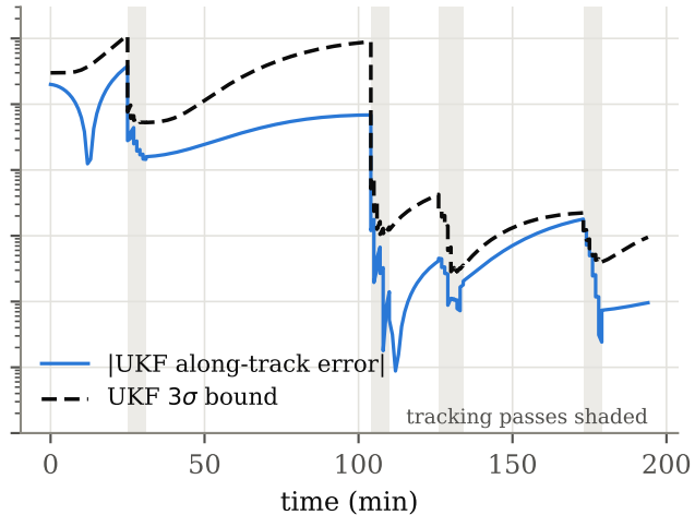
(b) UKF
