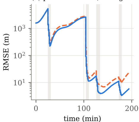
(c) position RMSE, TLE-grade
