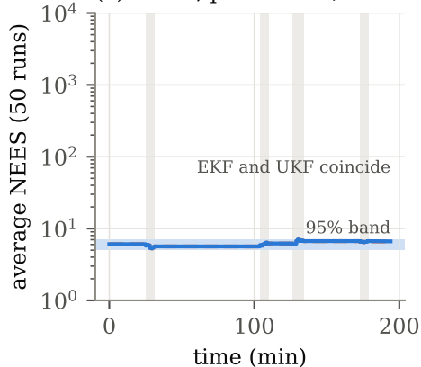
(a) NEES, prior 10 m / 0.01 m/s
