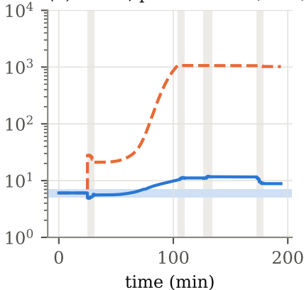
(b) NEES, prior 1000 m / 1 m/s
